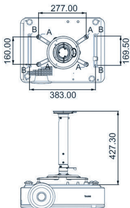
A: BenQ ceiling mount CMG3 (5JJAM10.001) Ceiling mount screw: M4 (Max. L = 25 mm; Min. L = 20 mm)
